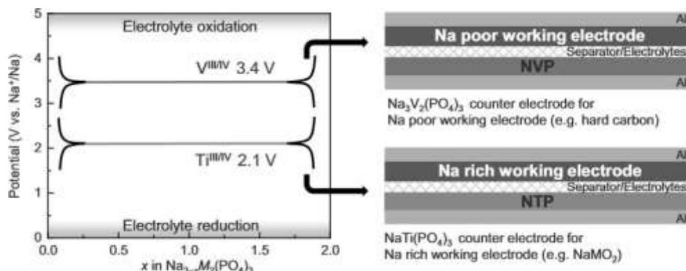
Figure 1. Concept of half-cell tests with NASICON counter electrodes.[6]
