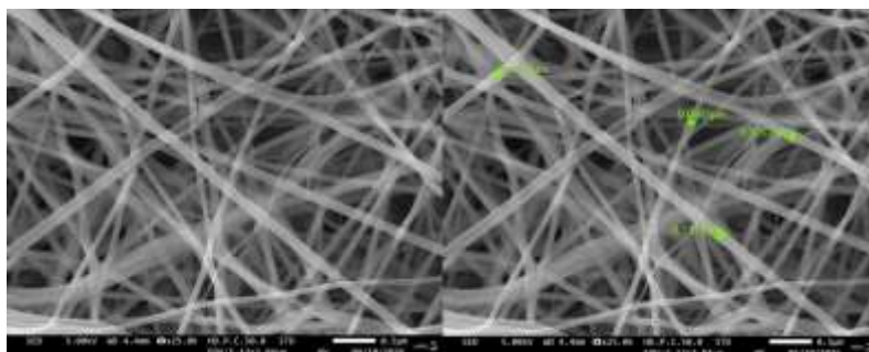
Figure 1. SEM images of the PVDF-HFP/LiClO 4 membrane .
