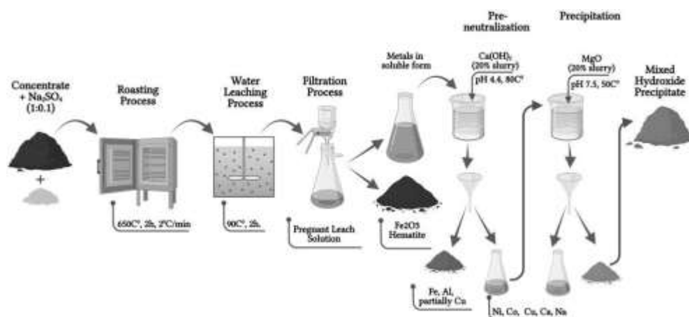
Figure 1. Experimental Flowsheet of the Four-Stage Hydrometallurgical Process for Conversion of Cu–Ni Sulfide Concentrate to MHP.
