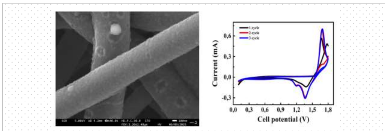
Figure 1. (a) SEM image and (b) CV curves of MnO 2 /PEDOT/PET nanofibers.
