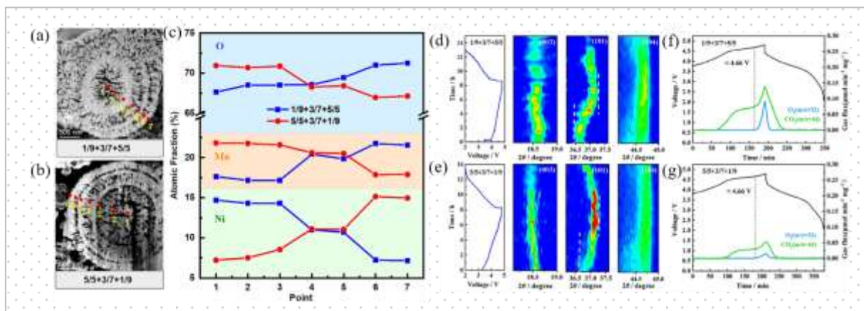
Figures 1 EDS elemental mapping analysis of a) 1/9+3/7+5/5 and b) 5/5+3/7+1/9 oxides illustrating 7 points locations. c) Elemental spot-scan analysis of O, Mn, Ni elements by taking 7 points from the center to the edge of 1/9+3/7+5/5 and 5/5+3/7+1/9 oxides. 2D contour plots of in situ XRD for d) 1/9+3/7+5/5 and e) 5/5+3/7+1/9 cathodes (0.2 C/2.0-4.8 V). Initial voltage profiles and gas evolution curves of CO 2 and O 2 for f) 1/9+3/7+5/5 and g) 5/5+3/7+1/9 samples (0.2 C/2.0-4.8 V)
