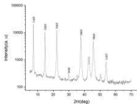
Fig.1 XRD patterns of the YBCO layer.
